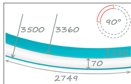
Motion Slim 3500 90°
