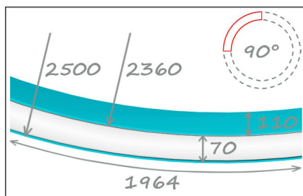
Motion Slim 2500 90°
