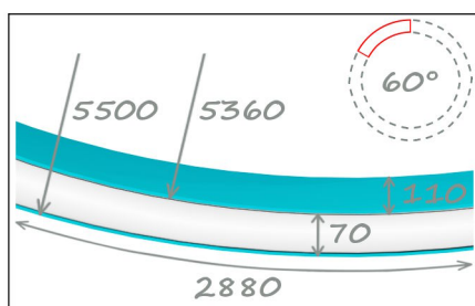
Motion Slim 5500 60°
